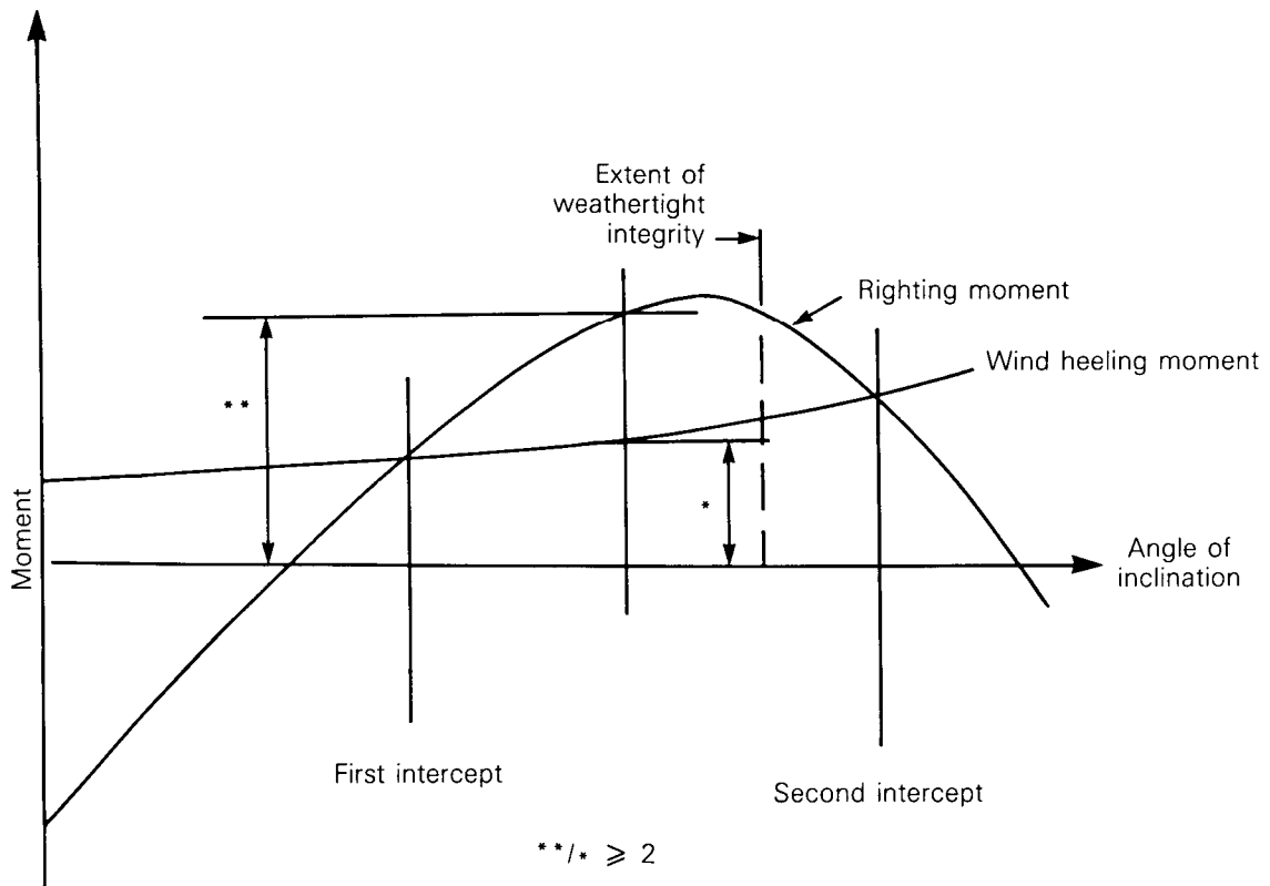
Figure 3-2 – Righting moment and wind heeling moment curves
