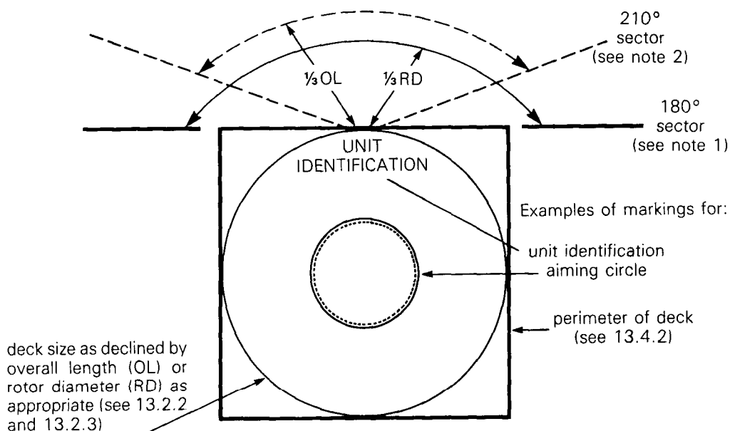
Figure 13-1 – Example of helicopter deck arrangement
