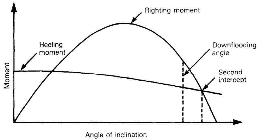
Figure 3-1 – Righting moment and heeling moment curves
